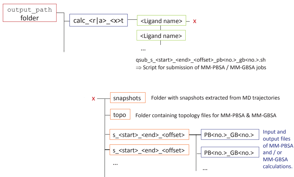
Figure 39.4.: Folder structure and files created during setup of MM-PB/GBSA calculations.
