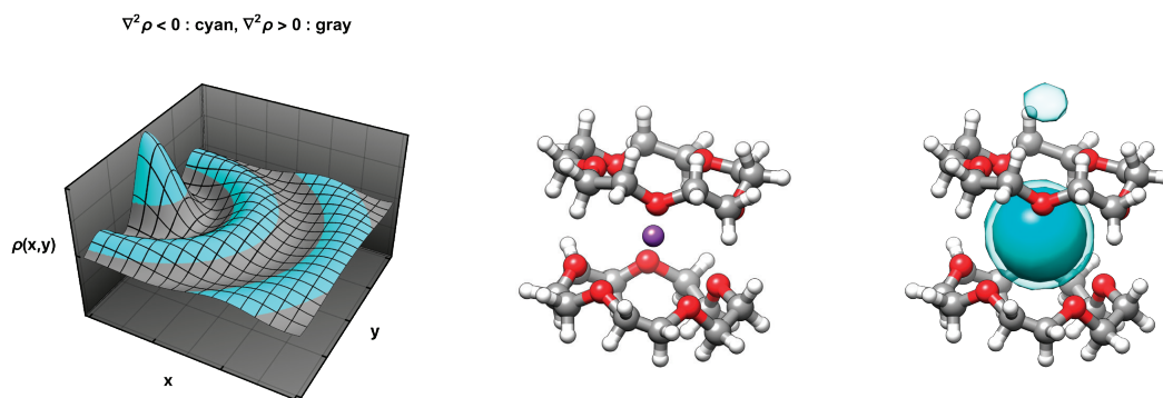
Figure 42.1.: (Left) The negative Laplacian (cyan) can be used to map locally concentrated regions of a density distribution, \rho . (Middle) A bis-crown ether (shown as CPK) binding mode to K^+ (violet sphere) determined using density distributions obtained using RISM and located using Laplacian mapping in MoFT. (Right) Two level sets of the Laplacian of the K^+ distribution, one using a threshold (see documentation) of 0.1 (solid cyan) and the other using a threshold of 0.01 (semi-transparent cyan).
