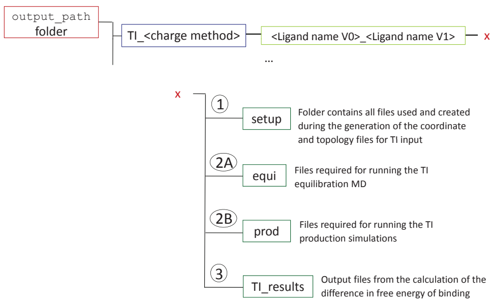
Figure 39.9.: Folder structure and files generated during TI calculation setup with FEW. Numbering according to steps shown in Figure 39.8.
