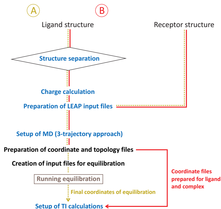
Figure 39.7.: TI workflow options: TI based on (A) a structure equilibrated using the MD setup functionality of FEW or (B) a user provided structure, e.g., a crystal structure.
