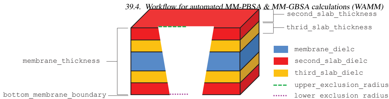
Figure 39.5.: Parameters for definition of implicit membrane in MM-PBSA calculations.
