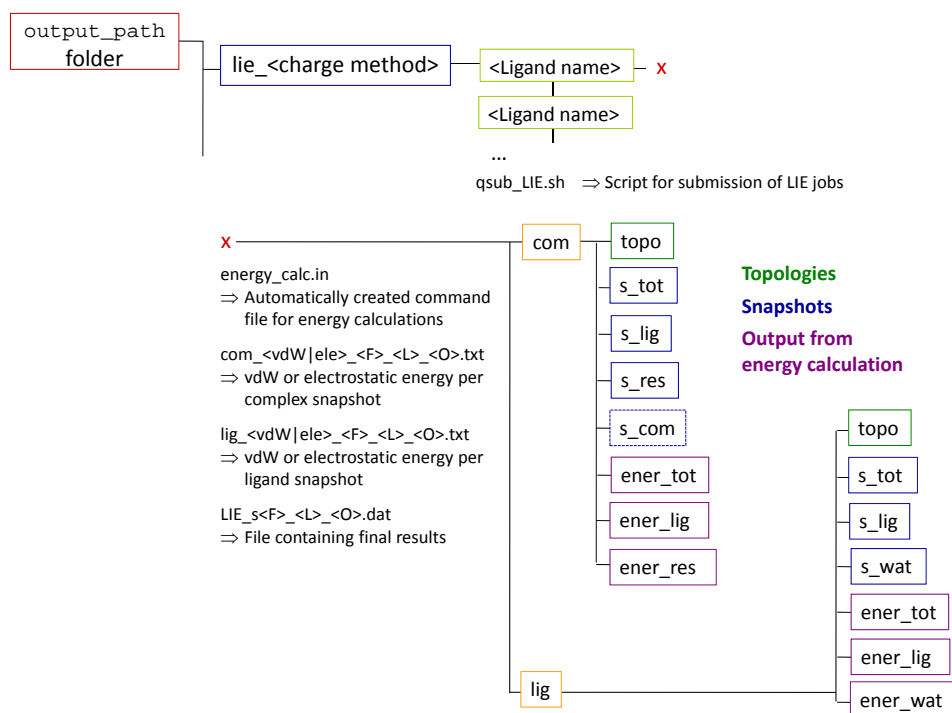
Figure 39.6.: Folder structure and files created during the setup of LIE calculations. For reasons of clarity first_lie_snapshot , last_lie_snapshot , and offset_lie_snapshots were replaced by aliases F , L , and O .
