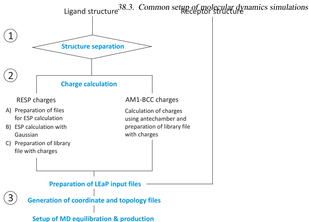
Figure 38.2.: Graphical illustration of the steps conducted for setup of MD simulations. Steps that can be executed independently by separate calls of FEW.pl are indicated by numbers. However, the individual steps can be combined, so that the whole MD simulation setup can be conducted in 1 or 2 steps for the AM1-BCC and RESP charge option, respectively (see 38.3).
