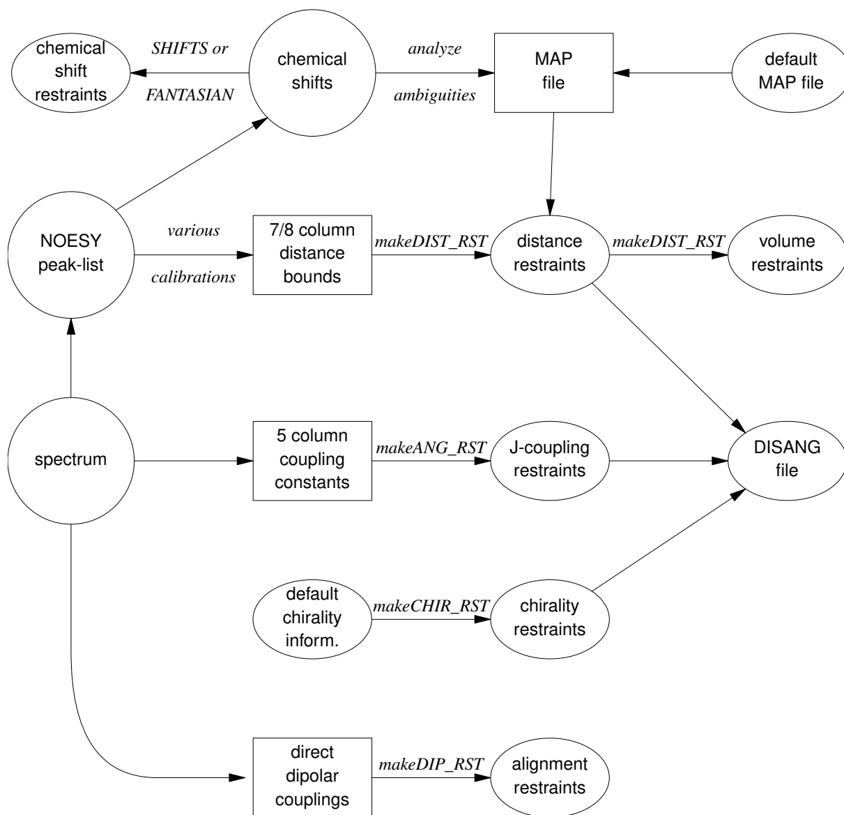
Figure 27.1.: Notation: circles represent logical information, whose format might differ from one project to the next; solid rectangles are in a specific format (largely compatible with DIANA and other programs), and are intended to be read and edited by the user; ellipses are specific to sander, and are generally not intended to be read or edited manually. The conversion of NOESY volumes to distance bounds can be carried out by a variety of programs such as mardigras or xpk2bound that are not included with Amber. Similarly, the analysis and partial assignment of ambiguous or overlapped peaks is a separate task; at TSRI, these are typically carried out using the programs xpkasgn and filter.pl
