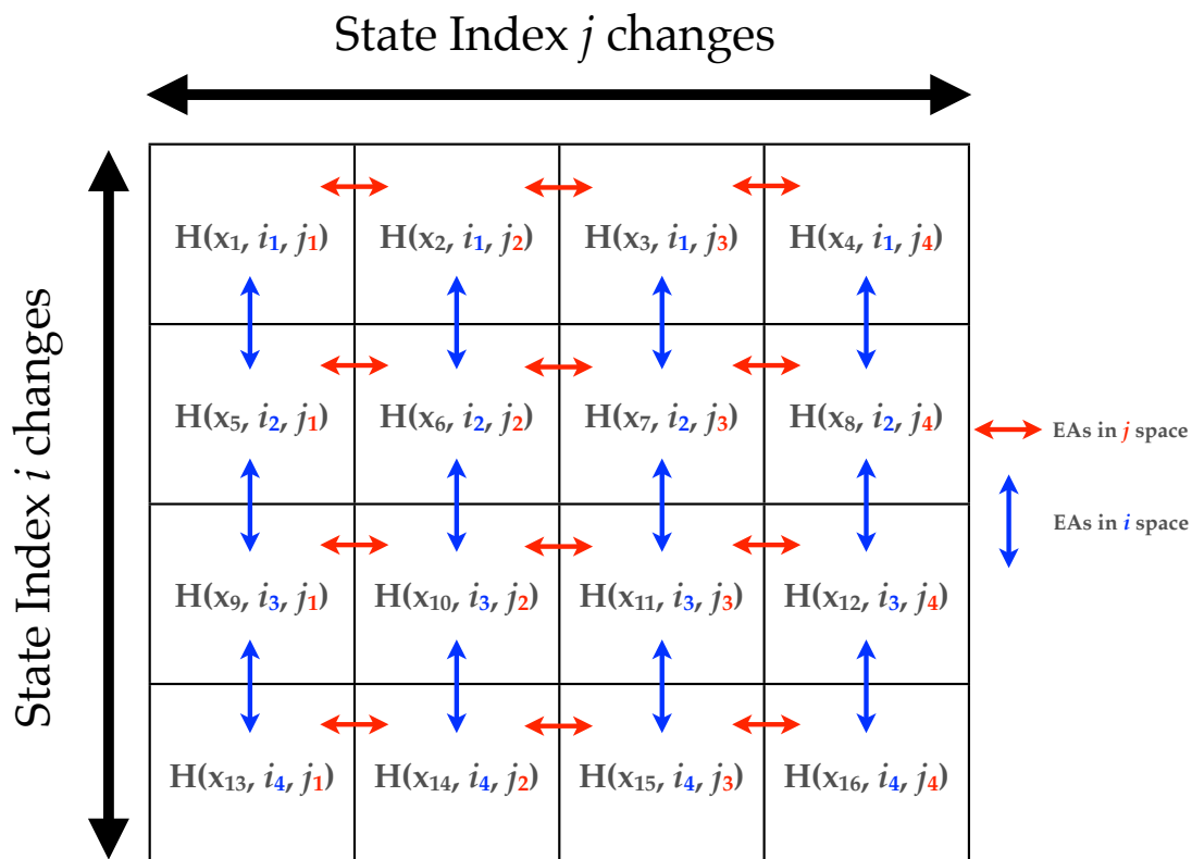
Figure 23.2.: Schematic showing exchange attempts (EAs) in multi-dimensional REMD simulations. Exchange attempts are indicated by the colored arrows, where red arrows indicate exchange attempts between replicas in a group of the dimension defined by the j state parameters. Blue arrows indicate exchange attempts between replicas in the dimension defined by the state parameter i . Figure taken from ref. 513.
