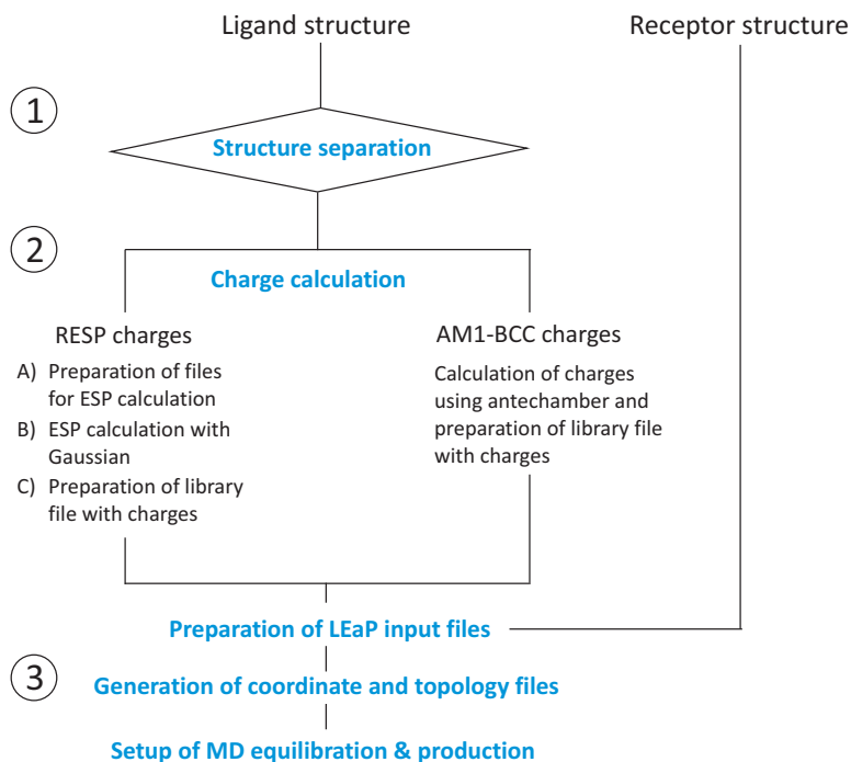
Figure 35.2.: Graphical illustration of the steps conducted for setup of MD simulations. Steps that can be executed independently by separate calls of FEW.pl are indicated by numbers. However, the individual steps can be combined, so that the whole MD simulation setup can be conducted in 1 or 2 steps for the AM1-BCC and RESP charge option, respectively (see 35.3).
