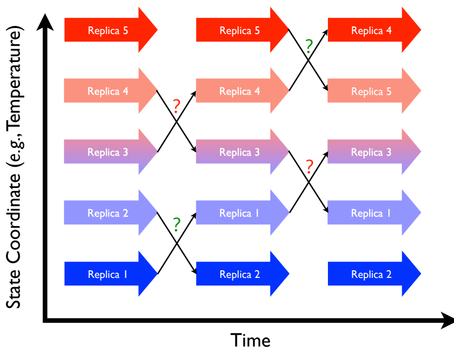
Figure 23.1.: Replica exchange schematic showing 5 replicas combined in an expanded ensemble. Large arrows represent MD trajectories of sub-ensembles while the smaller arrows represent attempted swaps between replicas in state space. Question marks represent Monte Carlo exchange attempts (green for successful, red for failed).
