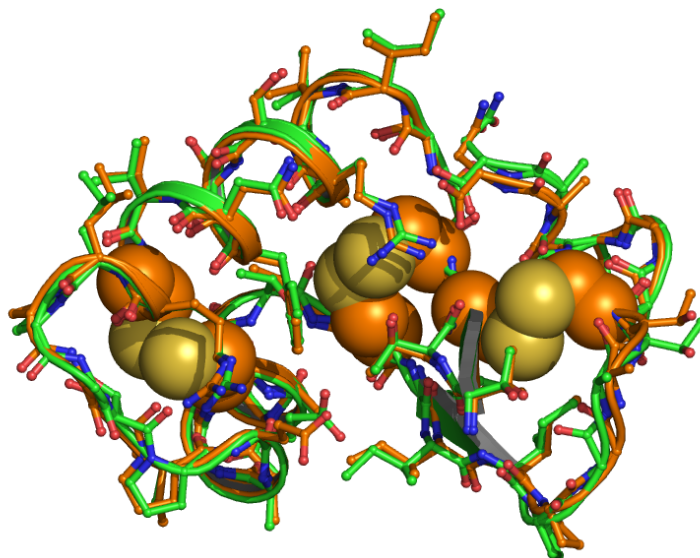
Figure 42.2.: Starting (green) and refined (orange) coordinates of 1CRN. Disulfide bonds in the refined structure are shown in CPK mode.
